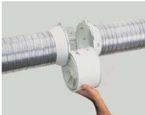
Simplified maintenance with slip out motor
